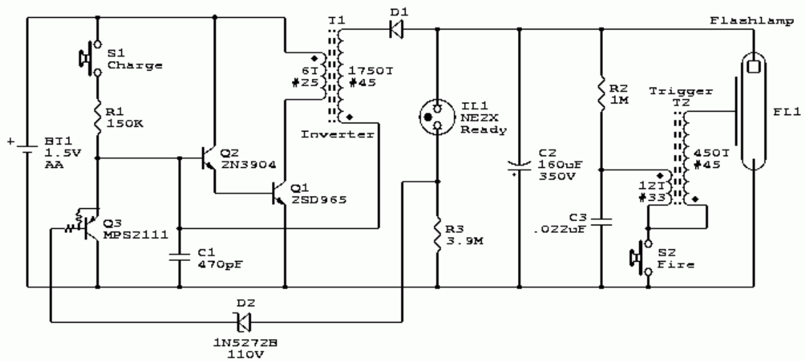
Kodak MAX Flash Unit
